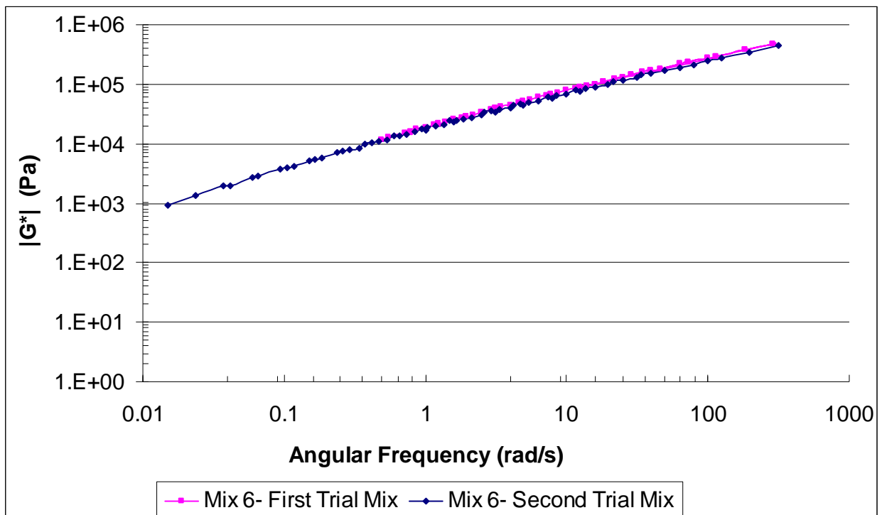
Figure 4.6. Repeatability of Binder Master Curve Determination
